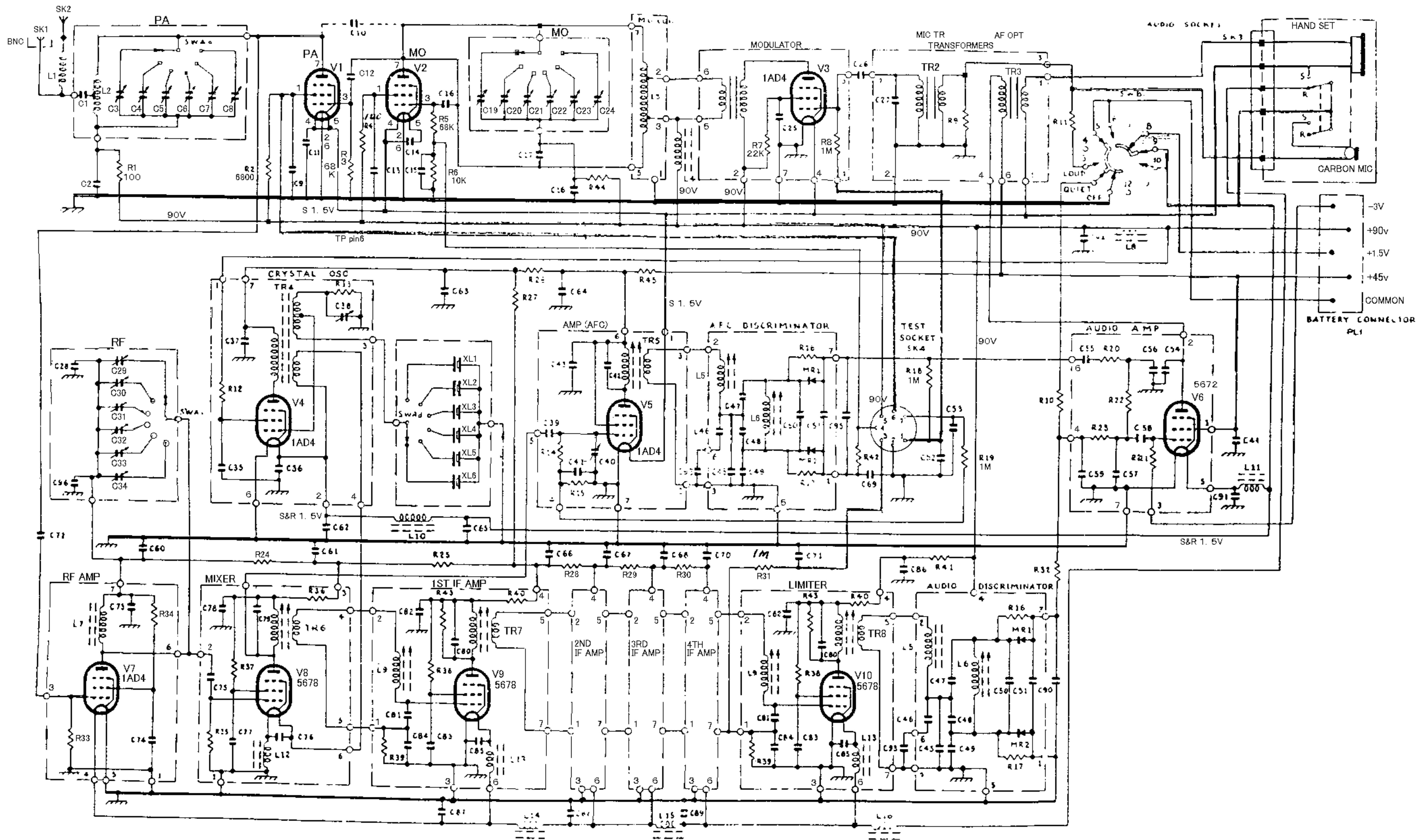
FIG. 1002 - MAIN SCHEMATIC WIRING DIAGRAM
